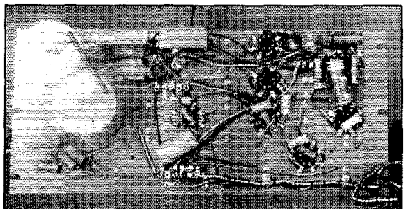
FRONT VIEW OF THE RECEIVER
