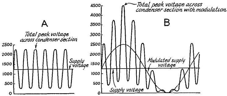
FIG. 2—VOLTAGES APPEARING ACROSS A CONDENSER SECTION OFF FIG. 1-B AND FIG. 1-C
