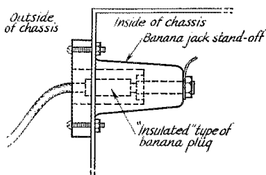
FIG. 2—NOVEL METHOD OF MOUNTING JACK-TOP INSULATOR TO AVOID EXPOSING "LIVE" PARTS
