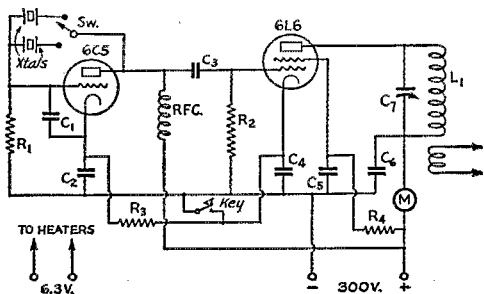
FIG. 1—WIRING DIAGRAM OF THE 6C5-6L6 PORTABLE-EMERGENCY TRANSMITTER
